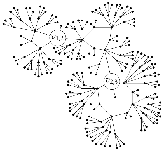
Figure 5. Structure of the graph H(4,6,8) with order 416, size 208 and degree sequence 1^{145}, 4^{52}, 7^9 .
