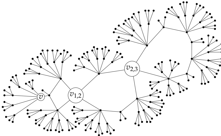
Figure 6. Structure of the graph T.H(4,6,8) with order 464, size 232 and degree sequence: 1^{162}, 4^{58}, 7^{10} .
