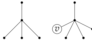
Figure 1. The tree T \cong S_6 where the vertex v is pendant.
