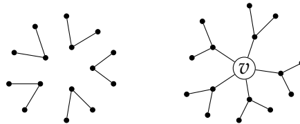
Figure 2. The tree T_2 with central vertex v connected to the centers of 5 copies of S_3 .
