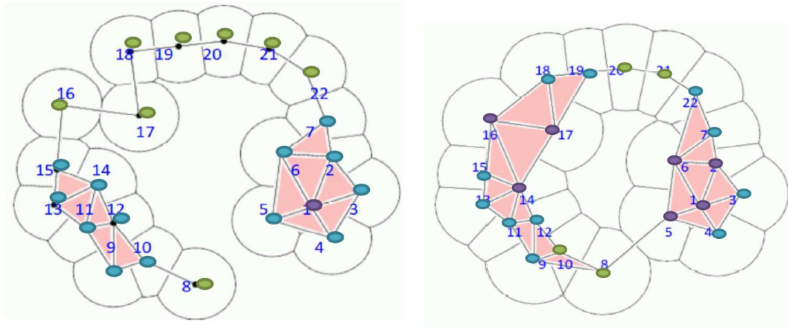
Figure 5. (left): graph V_1 , the sample cluster of galaxies whose graph depends from small Voronoi radius. (right): similar representation for graph V_2 based on larger small Voronoi disks. Both graphs show a good fit between the set of ordered values of \zeta_i (represented by colors) and their morphological role. Green indicate filament nodes, blue the wall, purple the cluster ones. In open graph like V_1 topological \zeta_i -sorting of nodes appears to work more efficiently.
